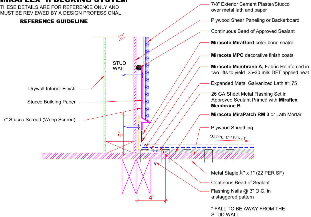
Plywood Substrate at Wood or Metal Stud Wall Detail #3B
